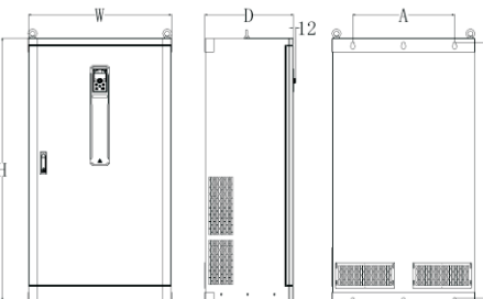
160KW Inverter Dimensions and Installation Dimensions
