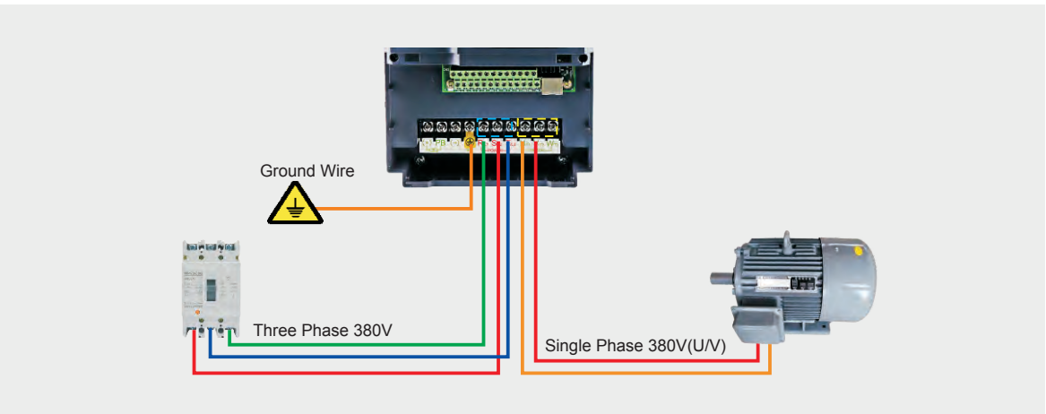
380V Single Phase Output Series
