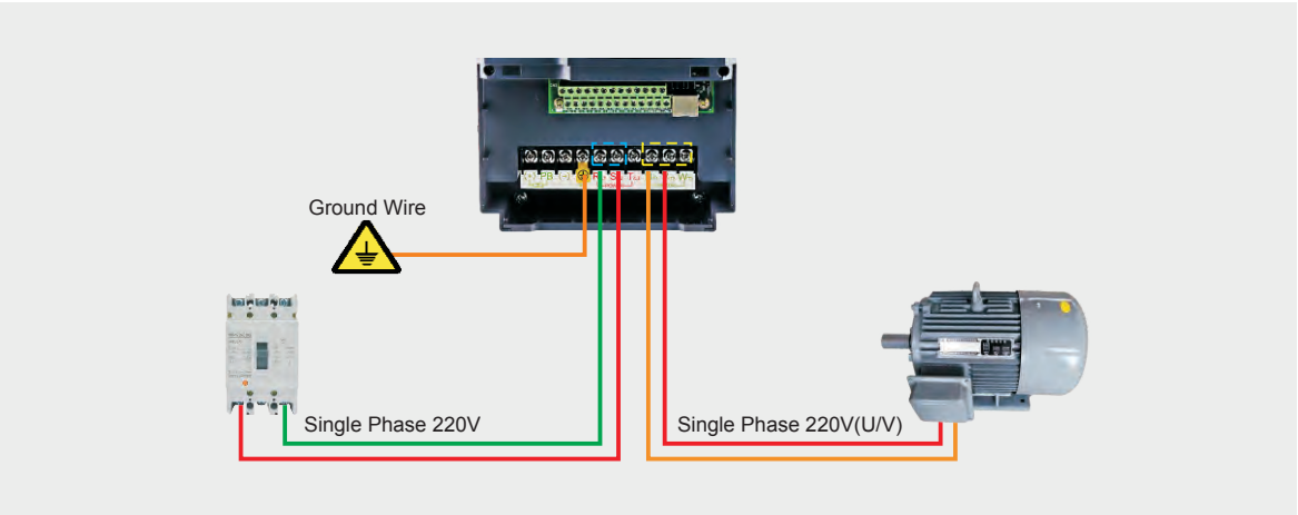
220V Single Phase Output Series
